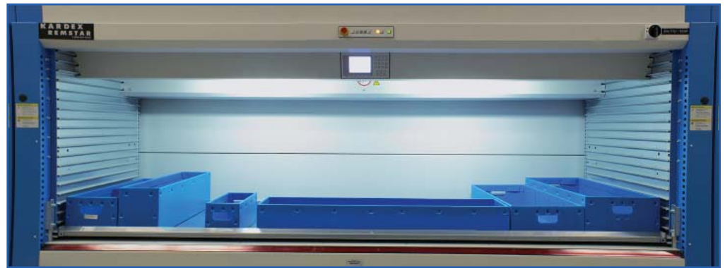
Interior of Remstar Vertical Shuttle. Shuttle trays are 3' x 10'. →
